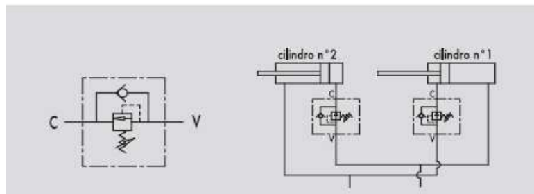
HYDRAULIC DIAGRAM
